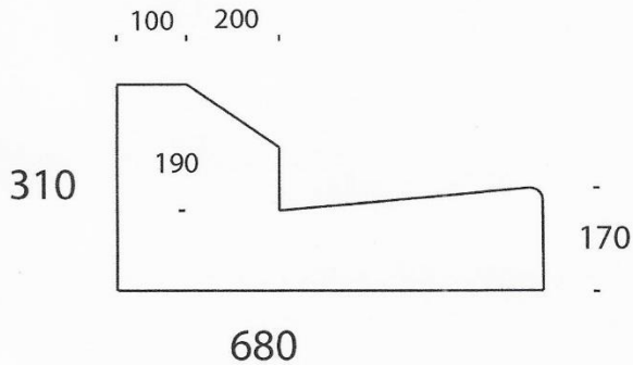
Large Kerb and Channel
