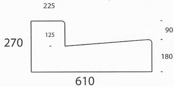
Hillside Kerb and Channel
