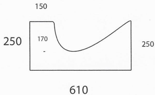
Kerb and Channel With Steel
