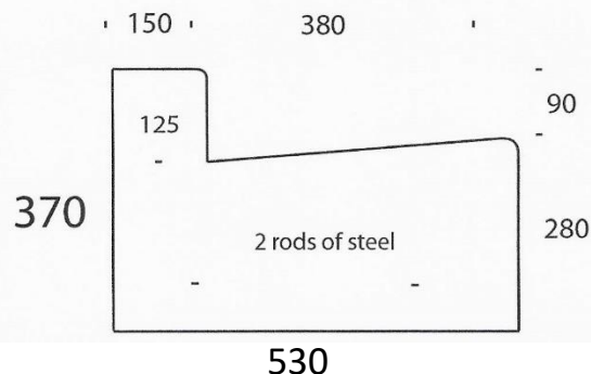
Kerb and Channel With Steel
