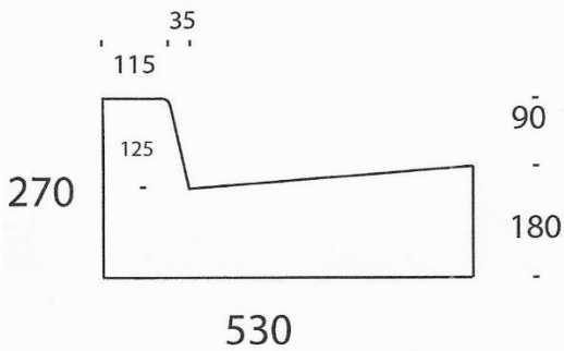
Sloping Kerb and Channel
