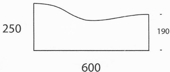
Kerb and Channel (shallow invert)
