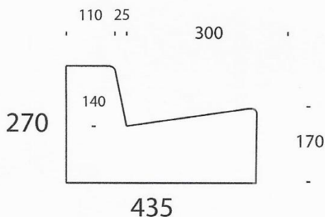
Kerb and Channel (narrow channel)
