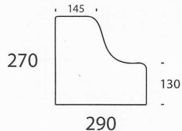
Kerb and Nib (2)
