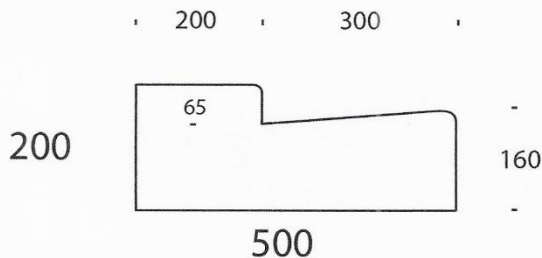
Kerb and Channel (shallow invert)
