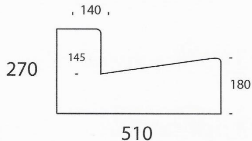
Kerb and Channel (deep Invert)
