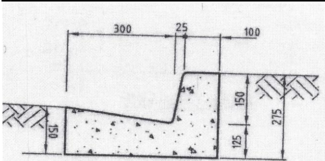
KERB & CHANNEL
