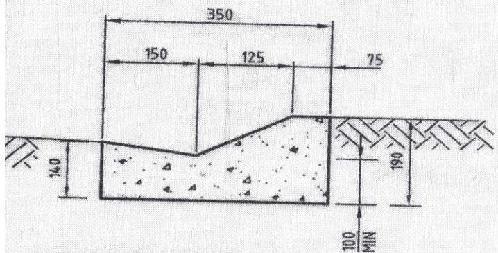
MOUNTABLE KERB & CHANNEL RESIDENTIAL
