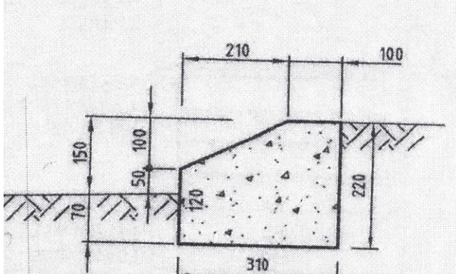
MOUNTABLE KERB
