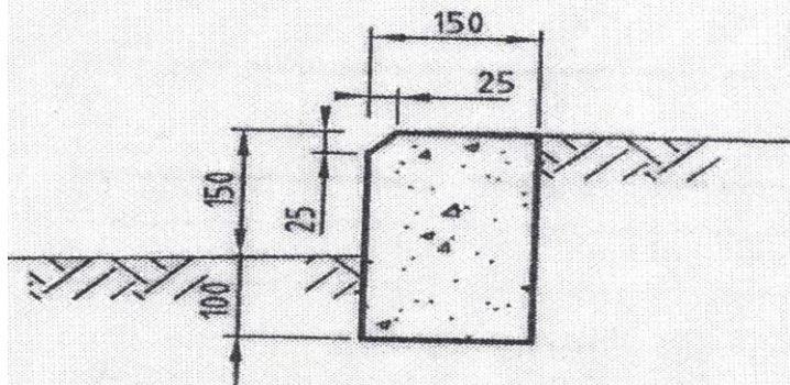
NIB KERB
