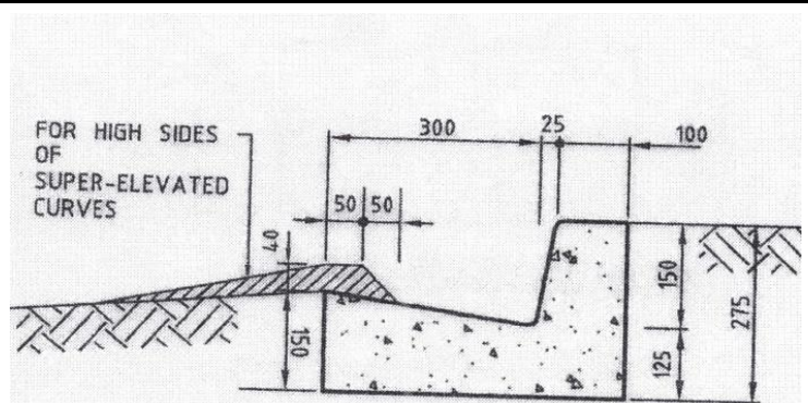
KERB & CHANNEL (SUPER ELEVATED CURVE)
