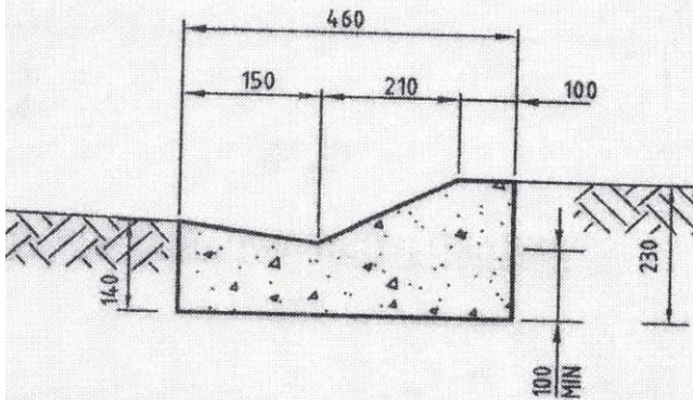
MOUNTABLE KERB & CHANNEL INDUSTRIAL & COMMERCIAL
