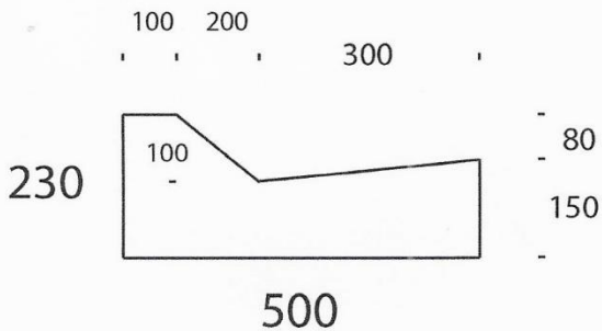
Cutdown Kerb and Channel (1)
