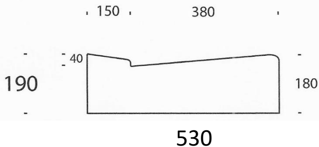
Cutdown Kerb and Channel (1)
