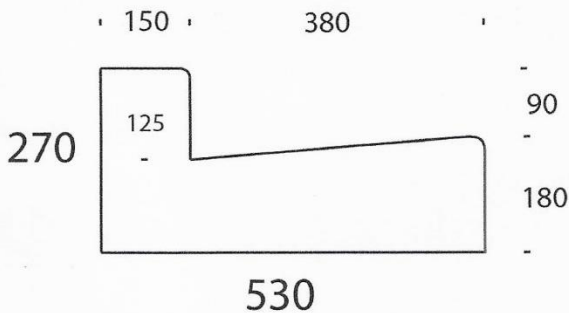
Low Profile Kerb and Channel
