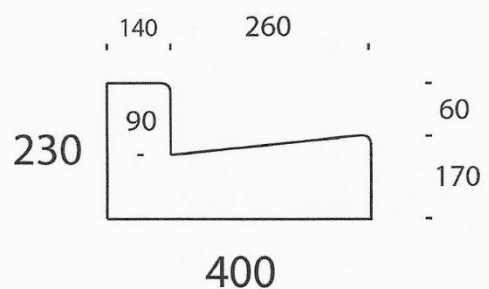
Timaru Kerb and Channel
