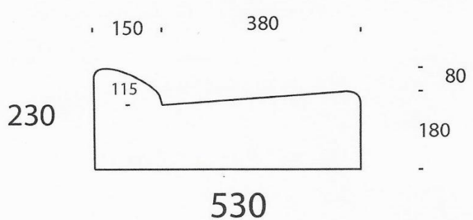
Small Kerb and Channel
