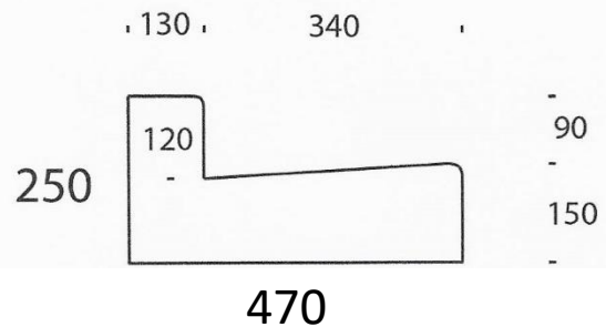
Timaru Kerb and Channel
