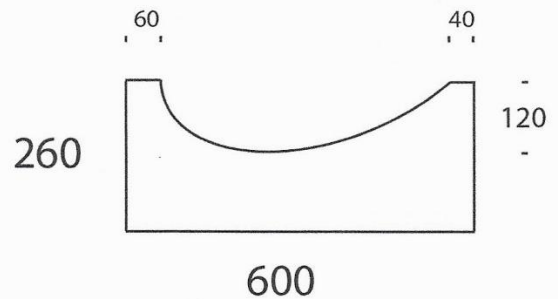
Off Set 600mm Dish Channel
