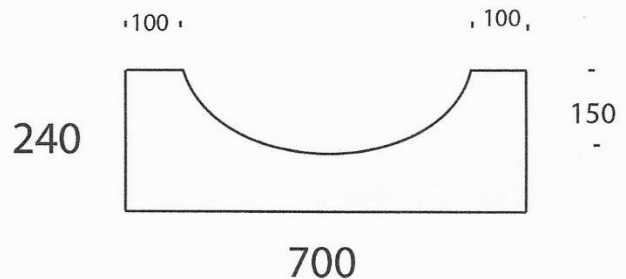
700mm Dish Channel
