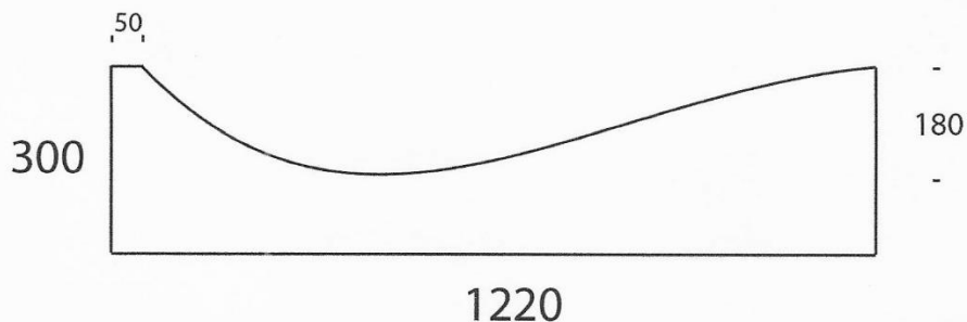
1220mm Dish Channel
