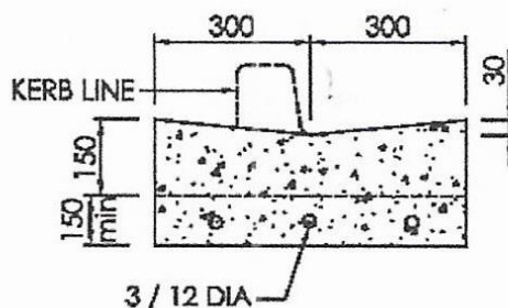
DISHED CHANNEL
