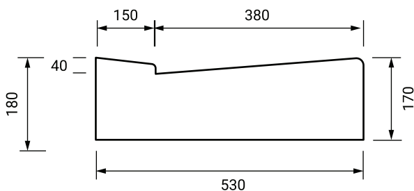
Cutdown Kerb and Channel
