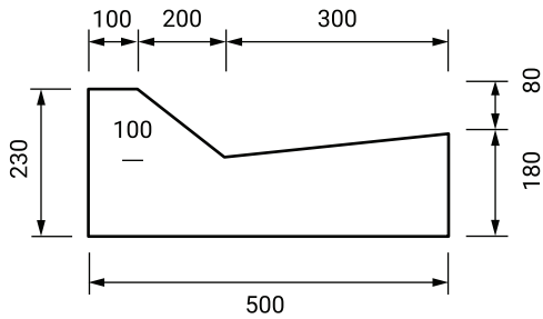
Low Profile Kerb and Channel
