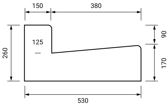
Kerb and Channel
