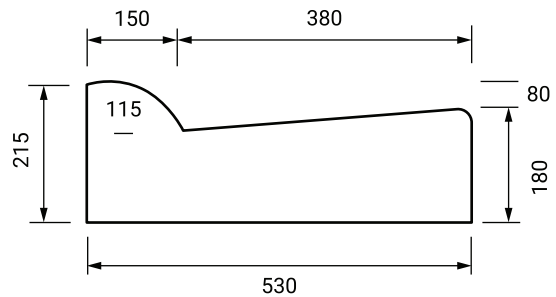
Low Profile Kerb and Channel
