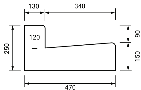
Timaru Kerb and Channel
