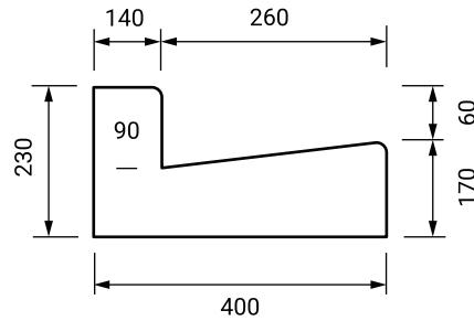
Small Kerb and Channel
