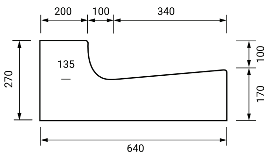
Large Kerb and Channel
