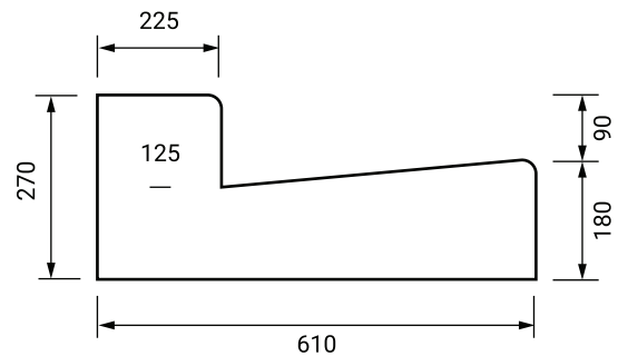
City Kerb and Channel
