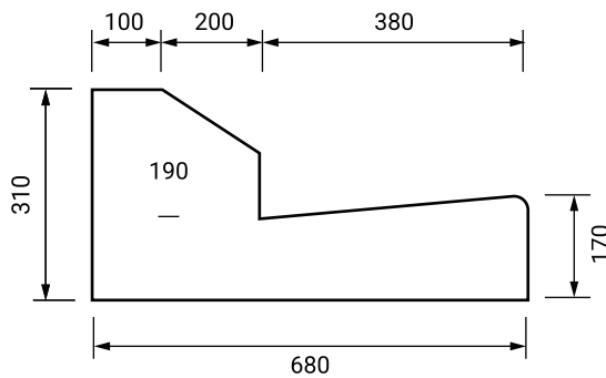
Mountable Kerb and Channel
