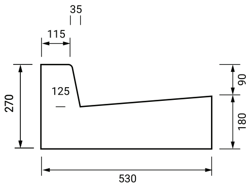
Sloping Kerb and Channel
