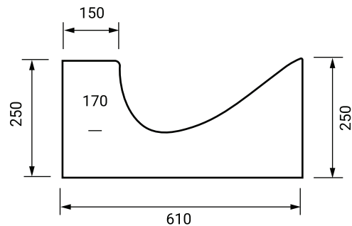
Hillside Kerb and Channel
