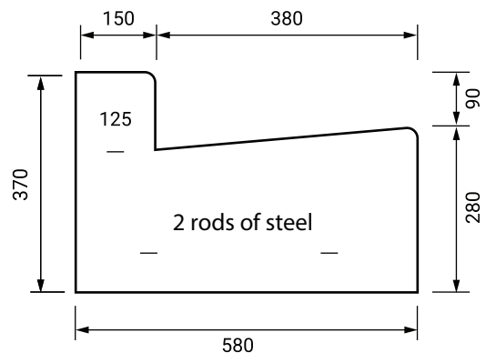
Kerb and Channel with Steel
