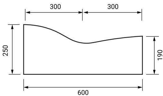
Roll Kerb and Channel
