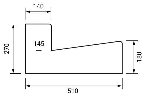
Kerb and Channel (Deep Invert)
