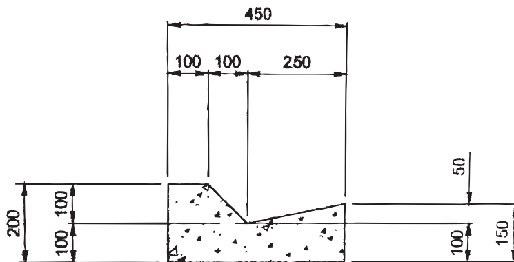
Kerb and Channel (Shallow Invert)
