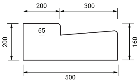
Kerb and Channel (Shallow Invert)
