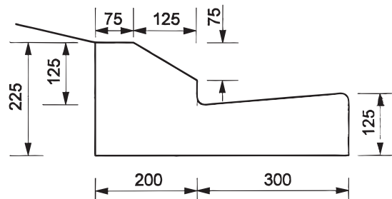
Mountable Kerb & Channel
