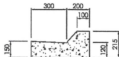
Kerb and Channel for Rural Edge Protection
