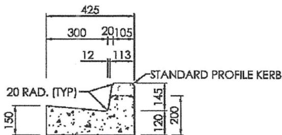
Machined Kerb and Channel
