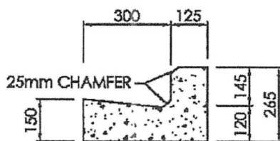
Boxed Kerb and Channel
