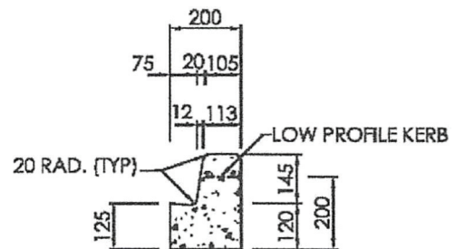
Machined Kerb Only
